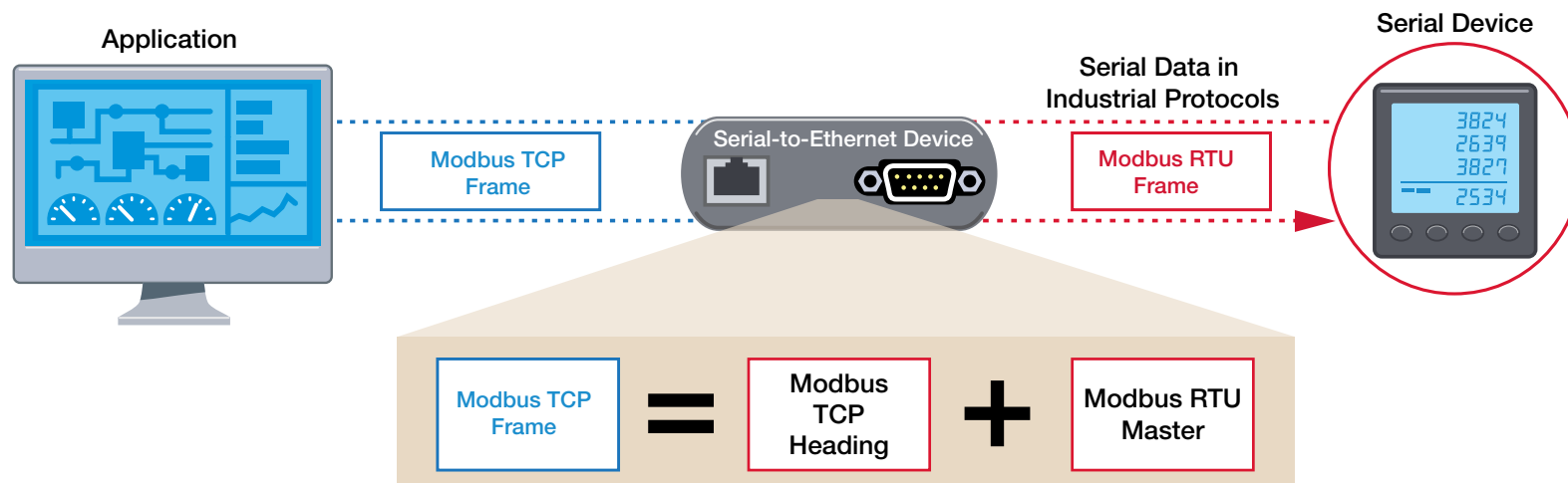
Figure 7: Serial-to-Ethernet communication: Transparent protocol conversion
